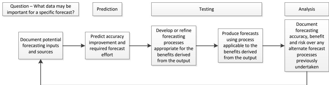
Figure 4: Forecasting Methodology
